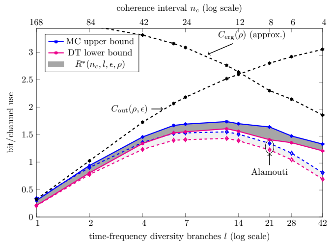
Fig. 3. m_t = m_r = 2 , n = 168 , \epsilon = 10^{-5} , \rho = 6 dB. Because of computational complexity, in the MC upper bound (35) the supremum over \{\Sigma_k\}_{k=1}^l is restricted to \{\Sigma_k\}_{k=1}^l of the form given in (51) when l > 7 .
