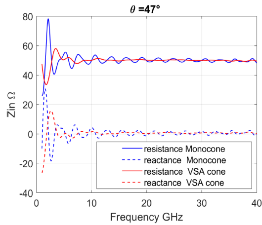
Figure 2: Simulated impedance comparison between classic monocone and VSA models
