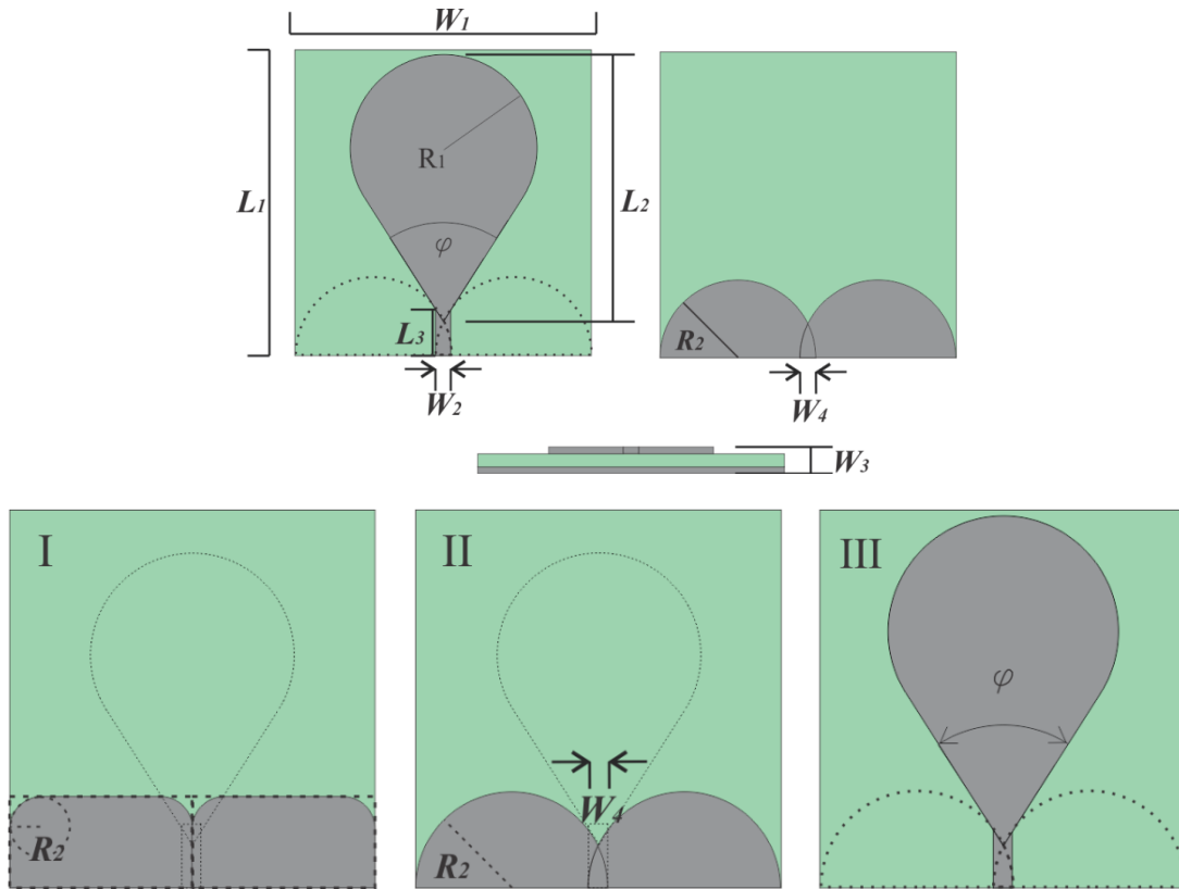
Figure 4: VSA MIMO unit cell and stages of the parametric study
