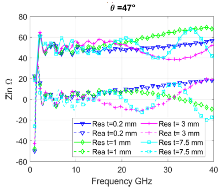
Figure 5: Input impedance ( Z_{in} ) analysis as a function of ground plane thickness for different configurations.
