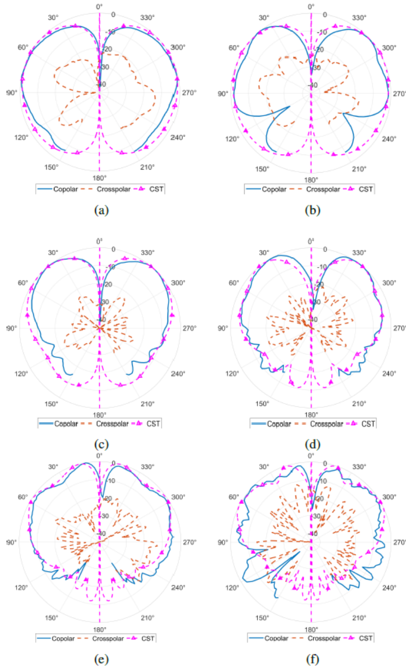
Figure 6: Radiation patterns at 1.7, 3.1, 6.85, 10.6, and 15 GHz for the 3D-VSA
