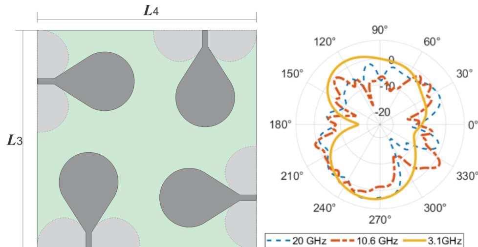
Figure 7: 2×2 MIMO Configuration and Far-Field Distribution at Three Key Frequencies
