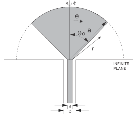
Figure 1: Cross-sectional view of the 3D-VSA design with curved ground plane
