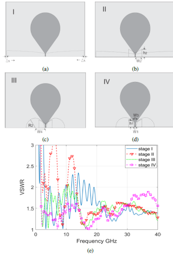
Figure 3: Optimization stages of the 2D-VSA design (I to IV)
