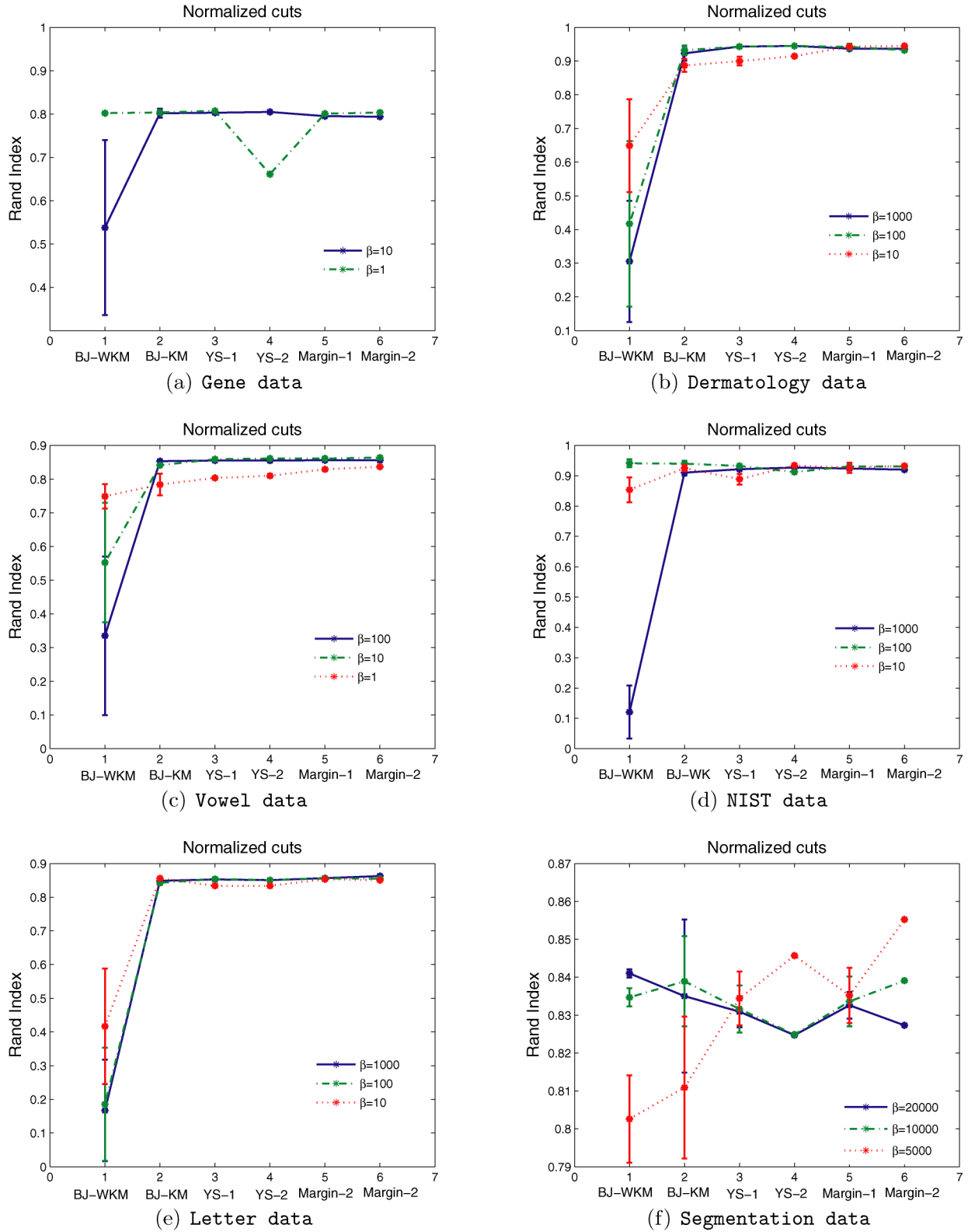
FIG. 2. Clustering results (Rand index) with normalized cuts. “BJ-WKM”: the weighted K -means rounding of Bach and Jordan 2006; “BJ-KM”: the K -means rounding of Bach and Jordan 2006; “YS-1”: the rounding scheme of Yu and Shi 2003 with the orthogonal initialization method; “YS-2”: the rounding scheme of Yu and Shi 2003 with initialization to the identity matrix; “Margin-1”: the rounding scheme in Section 3.1 with the orthogonal initialization method; “Margin-2”: the rounding scheme in Section 3.1 with initialization to the identity matrix.
